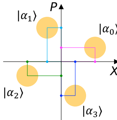
FIG. 1: Sketch of the four coherent states used to encode information.
