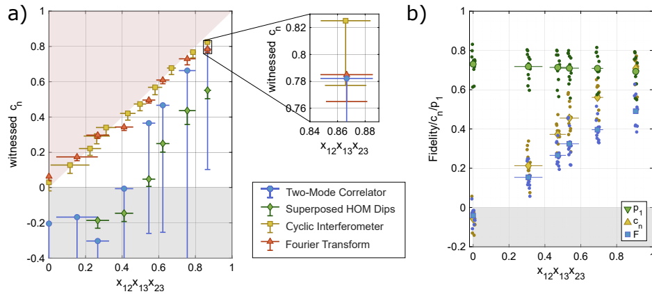
Figure 1: Experimental results. (a) Witnessed indistinguishability as a function of the product of pairwise overlaps of the internal states of 3 photons ( x_{1,2}x_{2,3}x_{1,3} ). Horizontal lines through the markers depict the standard deviation in x_{1,2}x_{2,3}x_{1,3} and the horizontal lines under the markers denote c_n(\varepsilon = 0.25) . The area that is marked gray witnesses no indistinguishability, and the area marked red has a higher indistinguishability than is allowed according to the theory. (b) Gate reversibility, indistinguishability, and fidelity witnesses for 12 Haar random 6-mode interferometers with \varepsilon = 0.1 .
