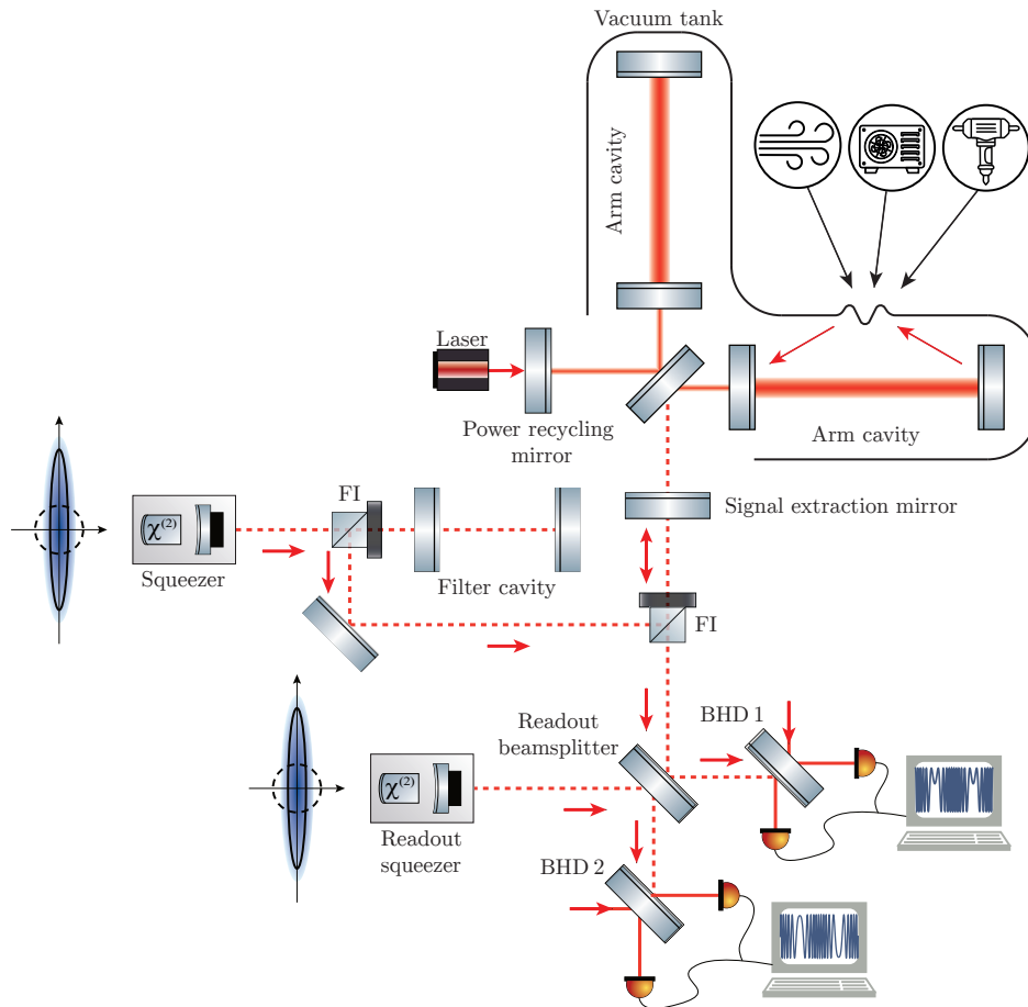
FIG. 1: Conceptual setup of our approach in a GW detector. The walls of the vacuum tanks are excited by microseisms and anthropogenic sources. Dual readout is implemented by the readout beamsplitter and two balanced homodyne detectors (BHD) in the output of the interferometer. One BHD measures the signal quadrature while the other one measures the witness quadrature. A second squeezed state is injected through the open port of the readout beamsplitter. Frequency-dependent squeezing is realized by a filter cavity and injected into the detector through a Faraday isolator (FI).
