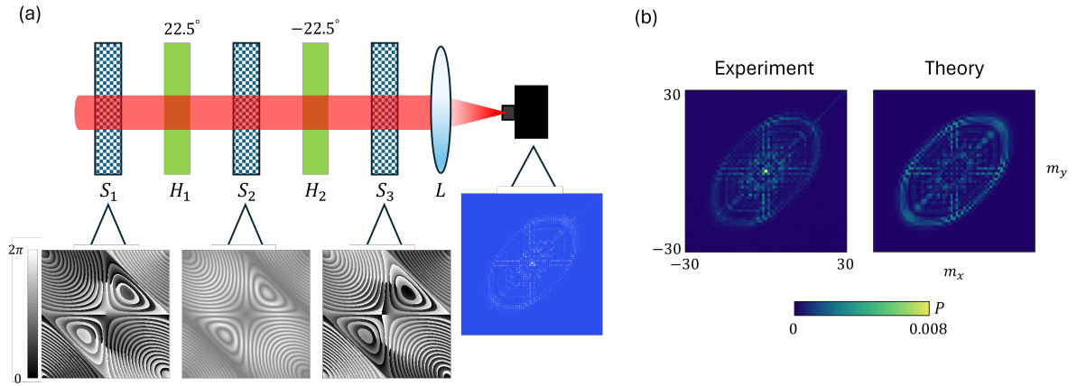
FIG. 1: (a) Experimental implementation of the reconfigurable three-SLM photonic circuit. The sequence of SLMs ( S_1 – S_3 ) and half-wave plates ( H_1 – H_2 ) implements a space-dependent polarization transformation whose output field maps into the evolved state of the target simulation. The displayed holograms correspond to a 30-step quantum walk on a two-dimensional lattice. (b) Measured output probability distribution for a 30-step two-dimensional quantum walk with a horizontally polarized input state, compared with the theoretical prediction.
