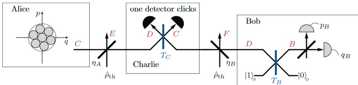
FIG. 1: Diagram of our setup from [4].
