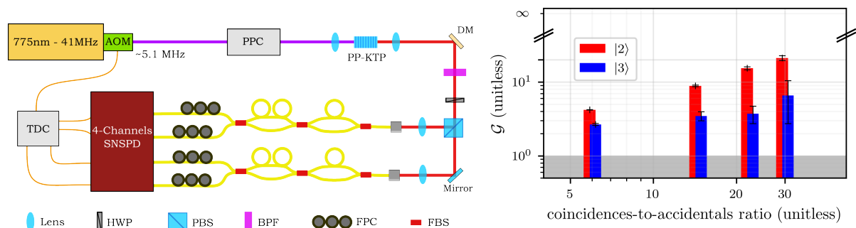
FIG. 1: (left) Experimental setup for preparing heralded states via waveguided PDC. (right) Ratio of the second- and third-order normalized moments \mathcal{G} = g^{(2)}/g^{(3)} in terms of the coincidences-to-accidentals ratio of the underlying photon-pair creation process for the heralded two and three photons. Ideally, these take the values \mathcal{G} \rightarrow \infty and \mathcal{G} = 3 , respectively. The gray shaded area shows the classical region. Abbreviations: AOM = acusto-optical modulator; BPF = bandpass filter; DM = dichroic mirror; FPC = fiber-coupled polarization controller; FBS = fiber-coupled beam splitter; HWP = half-wave plate; PBS = polarising beam splitter; PPC = power & polarization control; PP-KTP = periodically-poled KTiOPO 4 waveguide; SNSPD = superconducting nanowire single-photon detector; TDC = time-to-digital converter
